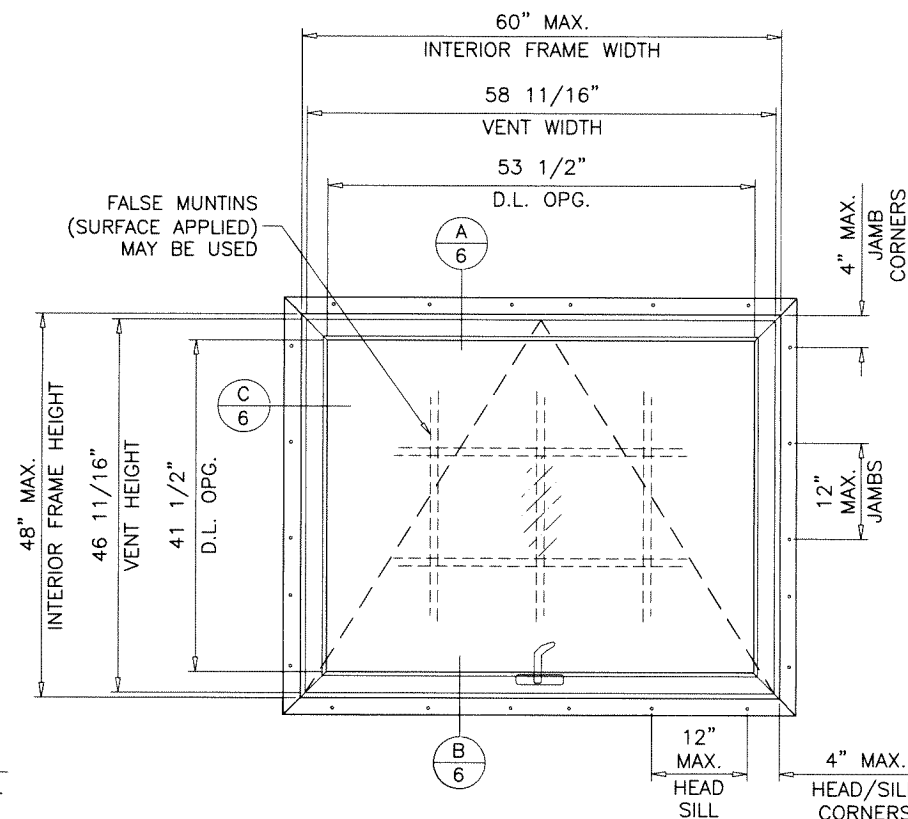
TYPICAL ELEVATION ANCHORS THRU NAIL FIN
